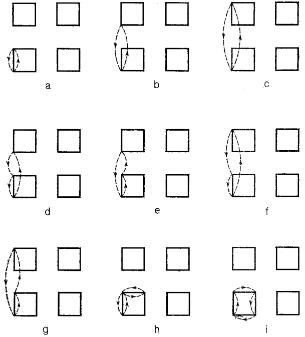
FIG. 4. Processes giving a contribution to E_0(\mathbf{k}) to order \beta^4 (for d = 2 ). The small squares positioned at the vertices of the large squares correspond to bands of the n th step of the renormalization group and are labeled by the index s ; their vertices correspond to the subbands, labeled by the index m , arising in the n th step. Transitions (s, m) \rightarrow (s', m') of the following form are taken into account: a) m' - m = \mathbf{e}_i , s' - s = 0 ; b) m' - m = 0 , s' - s = \mathbf{e}_i ; c) m' - m = \mathbf{e}_i , s' - s = \mathbf{e}_i . In the d -dimensional case the small and large squares are replaced by d -dimensional cubes.
